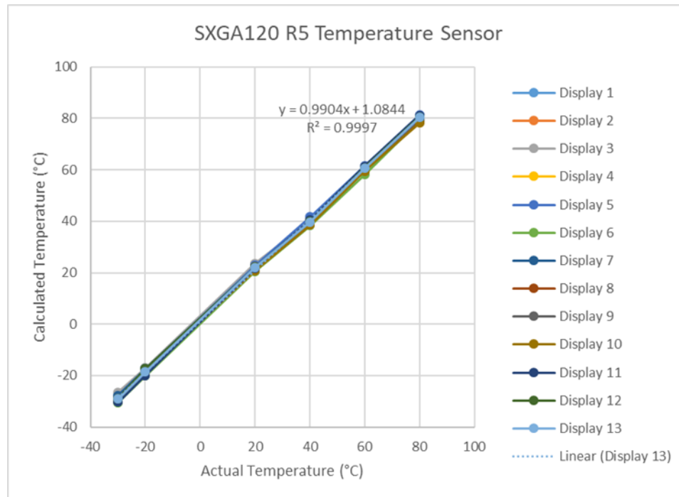
Figure 17 Measured Temperature vs. Actual Temperature
