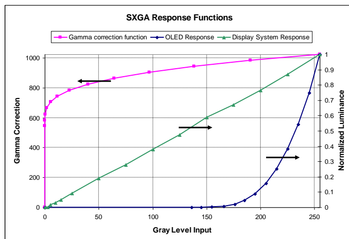
Figure 9: Gamma corrected system response characteristic
