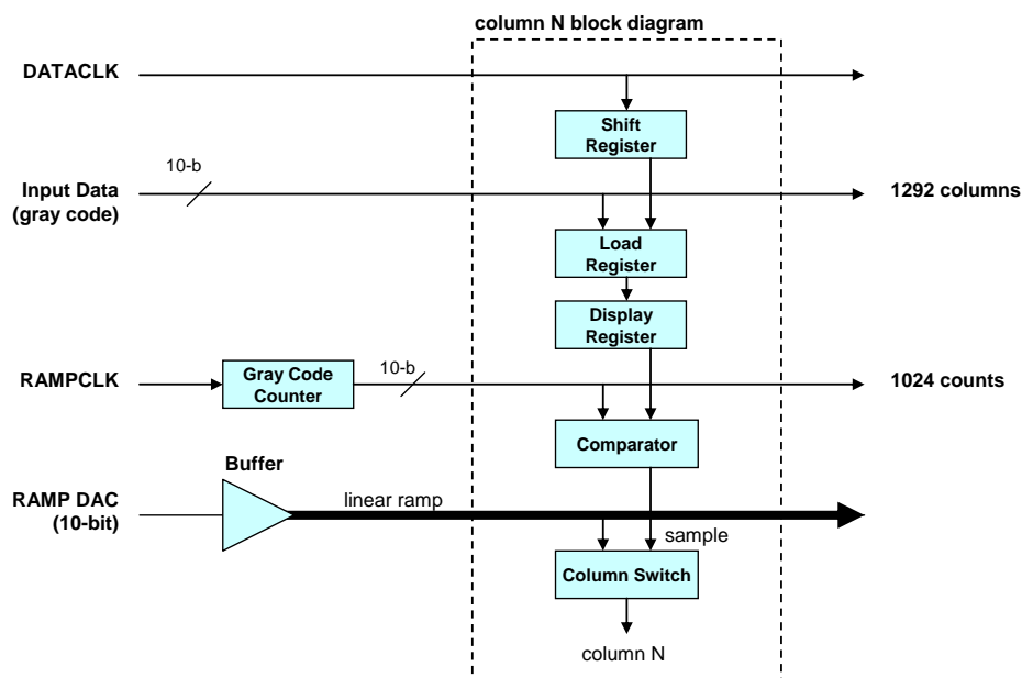
Figure 12 : Data sampling for Column N
