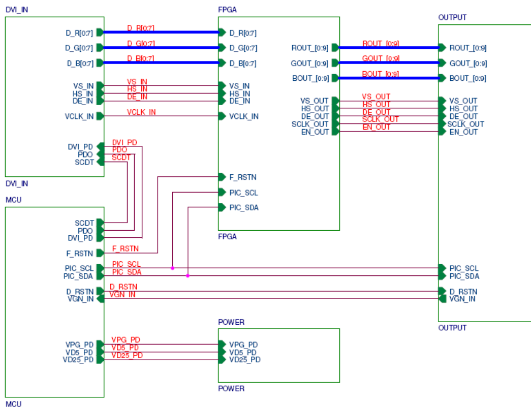
Figure 31 : Block diagram of application reference system
