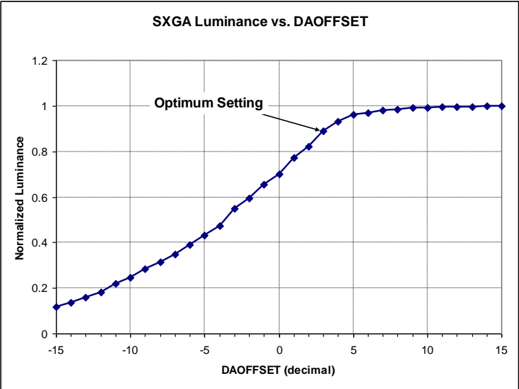
Figure 28: Luminance dependency on DAOFFSET
