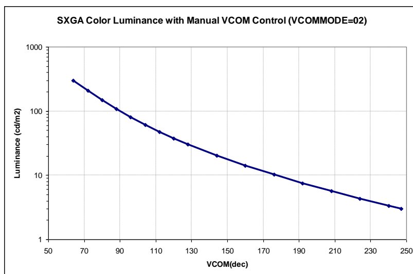
Figure 29: Typical luminance dependency on manual VCOM setting
