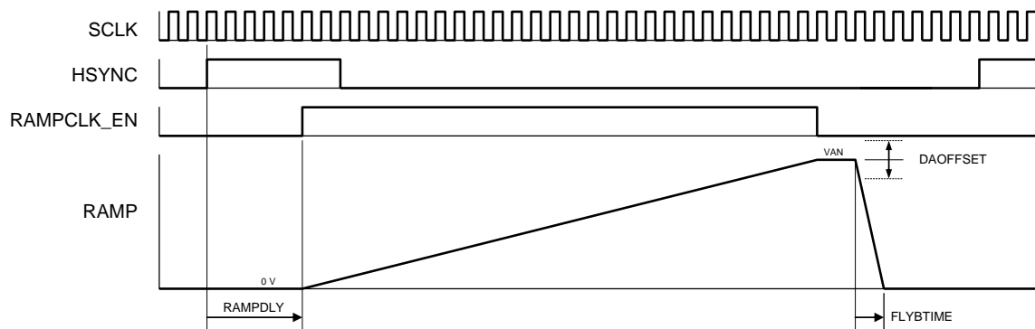
Figure 13 : Timing diagram for column data sampling
