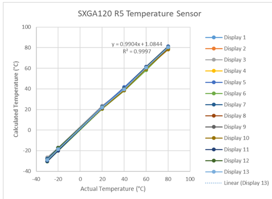
Figure 17 below illustrates the correlation between measured (calculated with the above formula) and actual ambient temperature.
