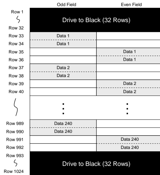
Figure 14 : Interlace option showing VGA mode with line doubling
