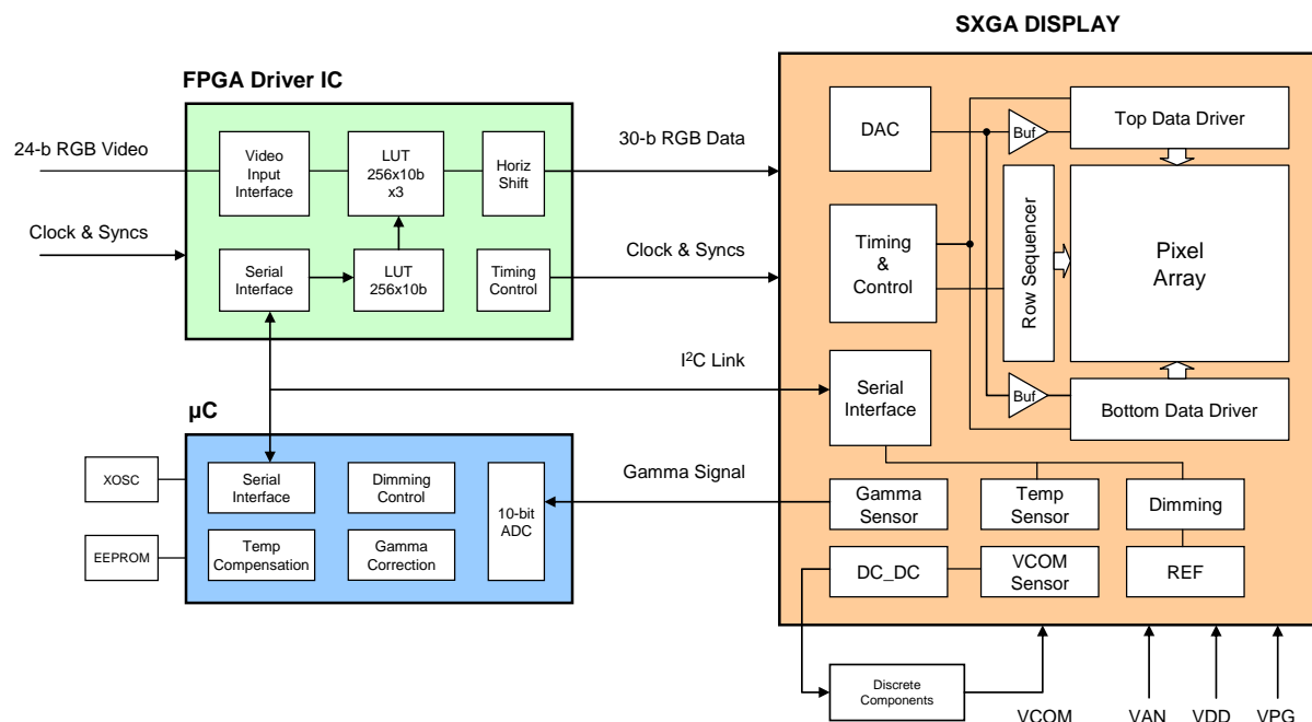
Figure 31 : Block diagram of application reference system
