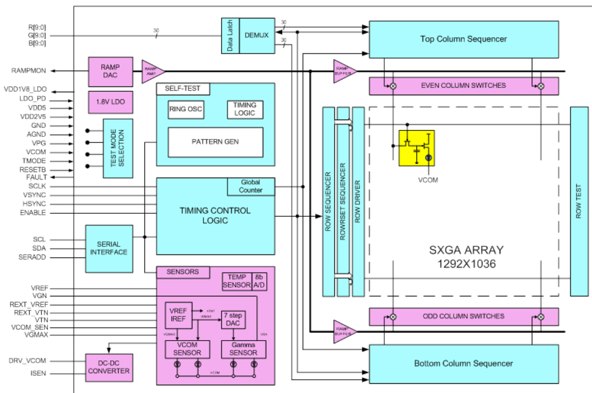
Figure 1 : SXGA120 design block diagram
