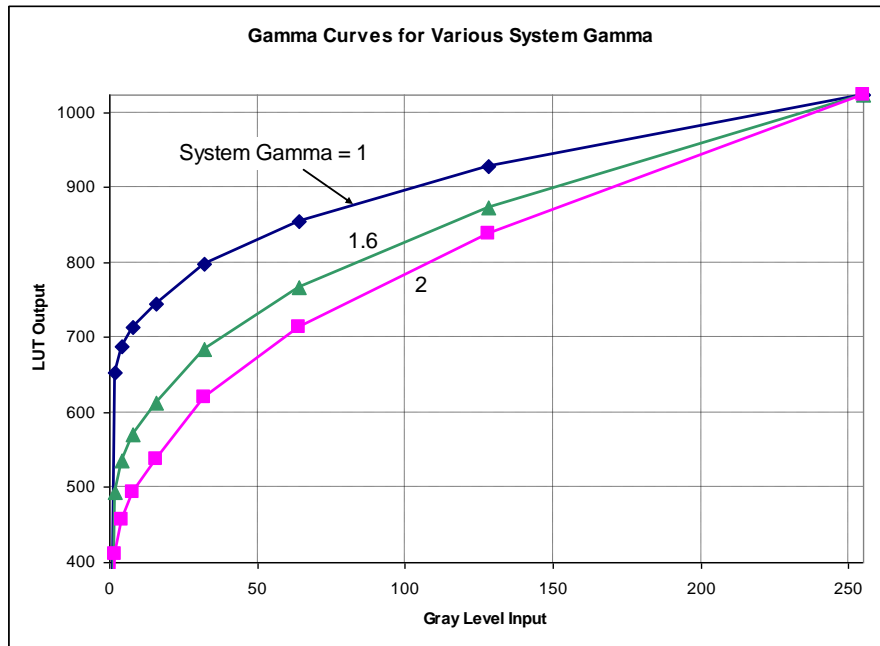
Figure 22 : Gamma curves for arbitrary System Gamma
