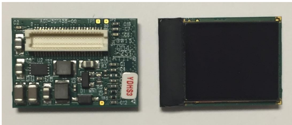
Figure 34: Photo of Microdisplay Assembly (A01-501458-00)
