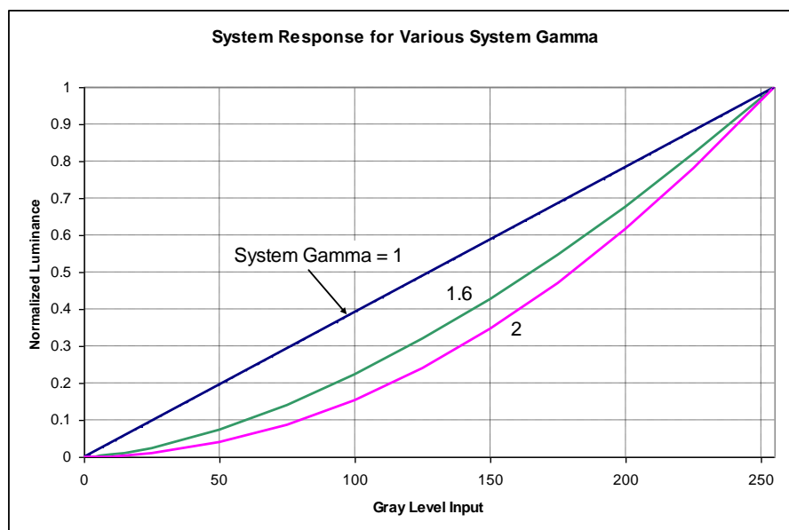
Figure 23 : Display system response for arbitrary system gamma
