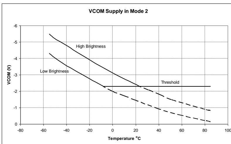
Figure 25 : VCOM supply characteristic in Mode 2
