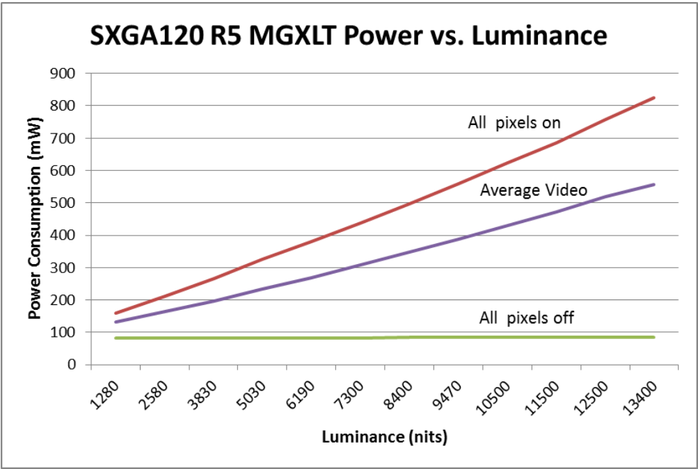
Figure 2 : Total power consumption vs. luminance at 20°C – SXGA120 R5 MGXLT
