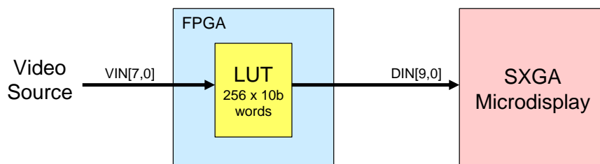
Figure 10: Gamma correction using a look-up-table (LUT)
