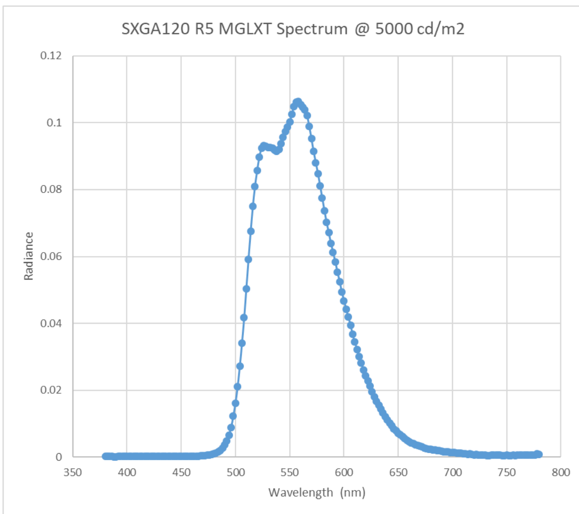
Figure 4: Spectral Response
