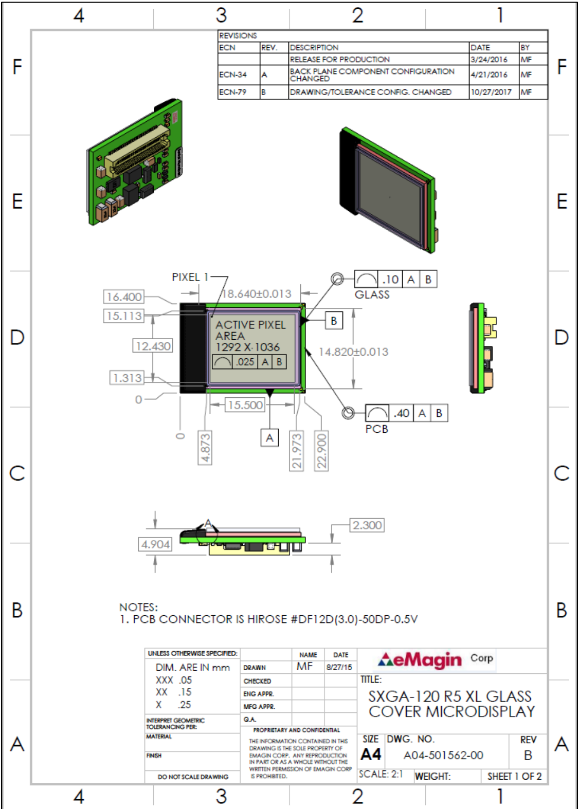
Figure 5: SXGA Assembly Drawing with 0.7mm Glass Cover (A04-501562-00)
