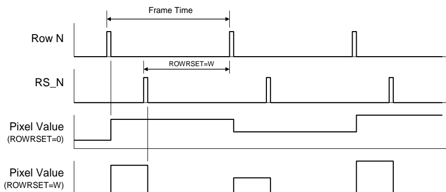
Figure 16: Timing diagram showing Row Reset functionality
