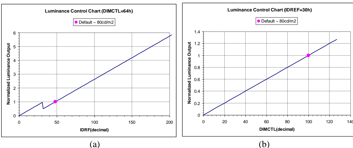
Figure 18 : Typical maximum luminance for various IDRF (a) and DIMCTL (b) settings
