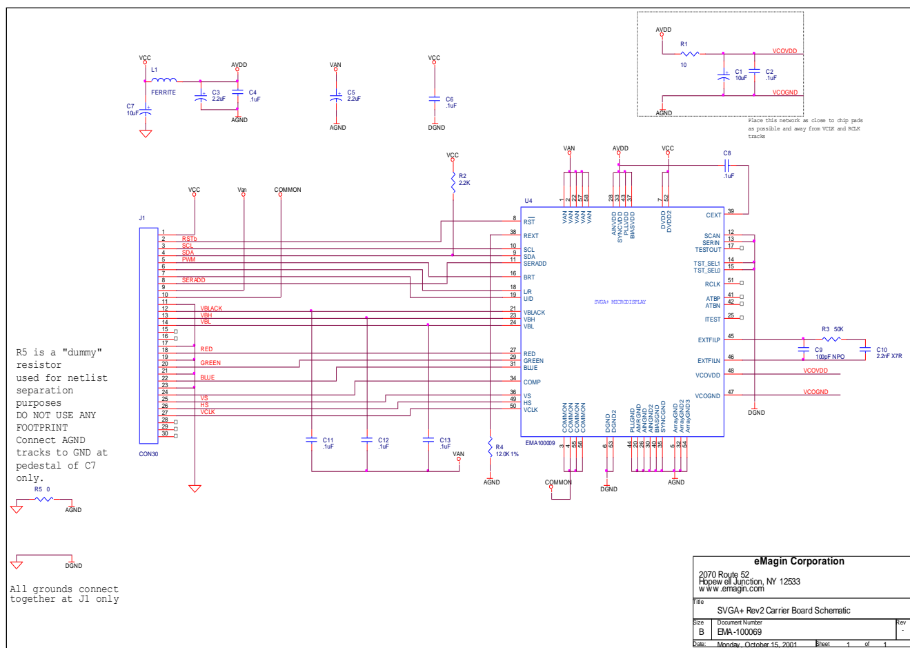
Figure 13-1. Microdisplay Carrier Board Electrical Diagram
