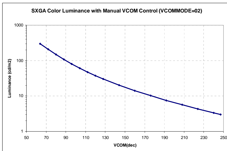
Figure 18: Typical luminance dependency on manual VCOM setting
