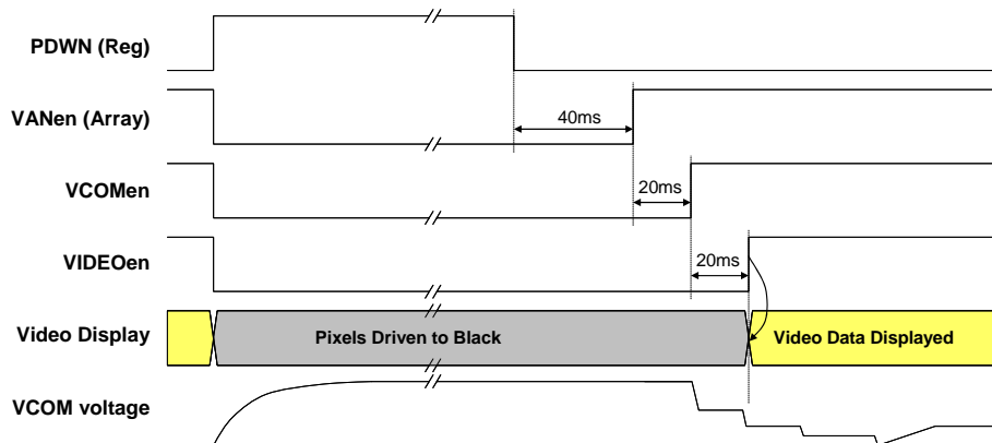
Figure 18 : Soft power-down / power-on sequence for supplies and control.
