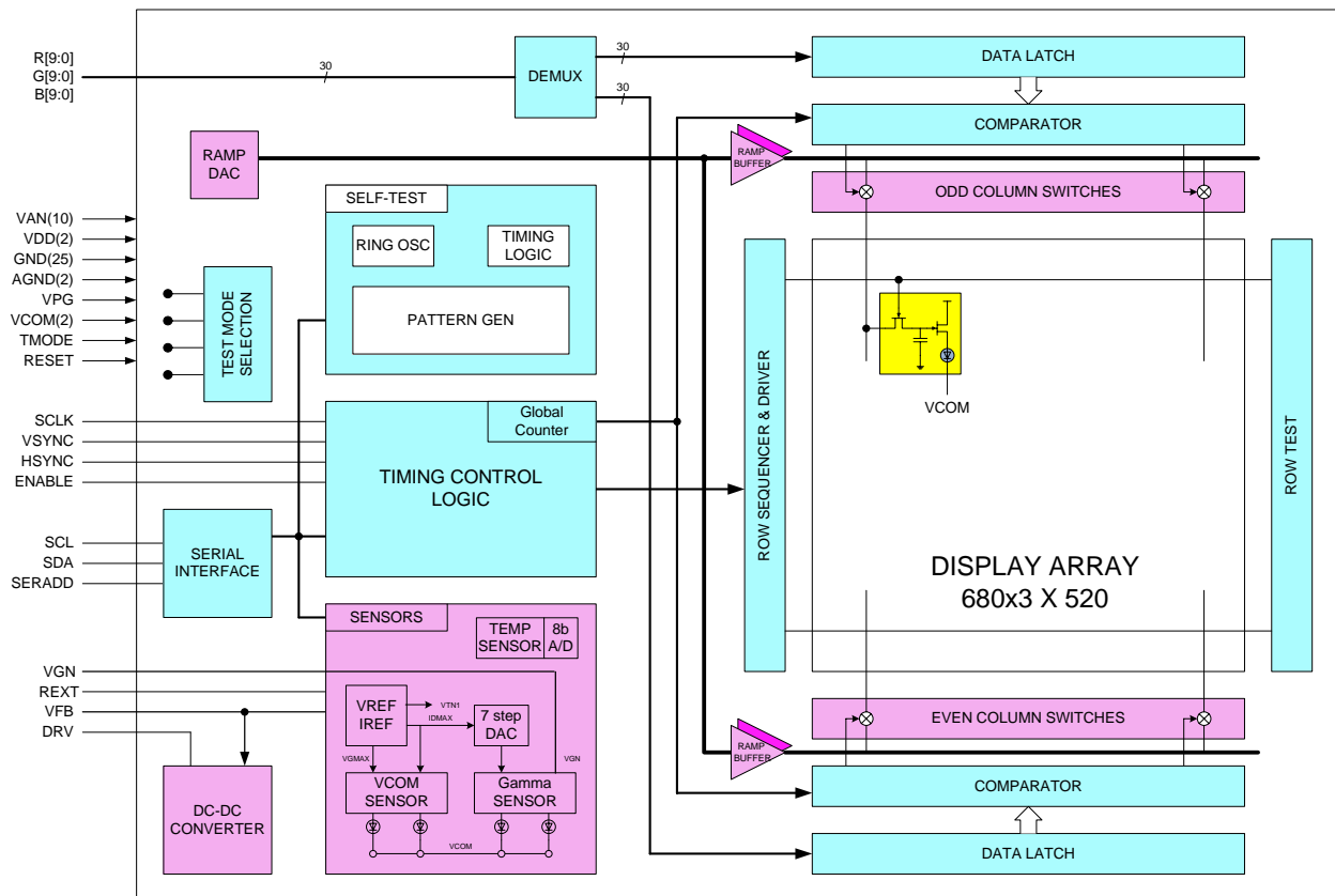
Figure 1 : VGA design block diagram
