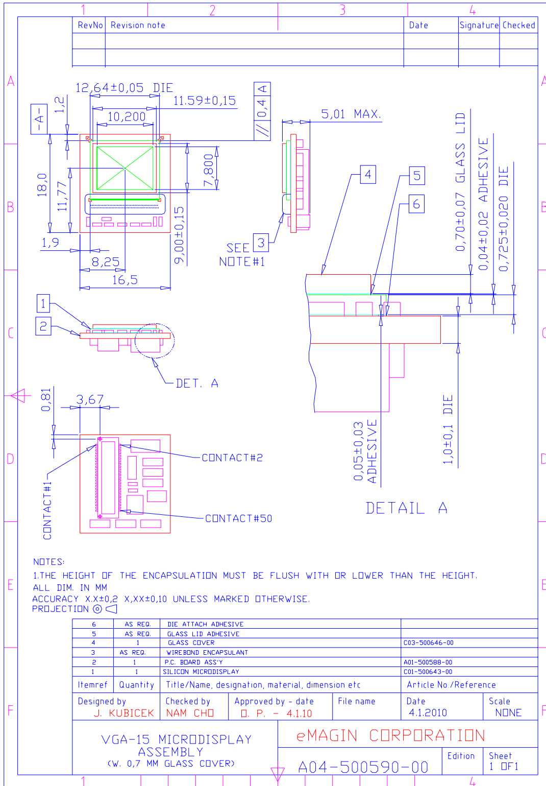
Figure 3: Color VGA Microdisplay IC Drawing with 0.7mm Glass Cover
