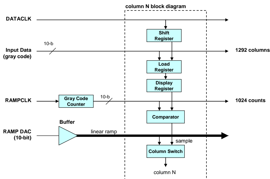
Figure 7 : Data sampling for Column N
