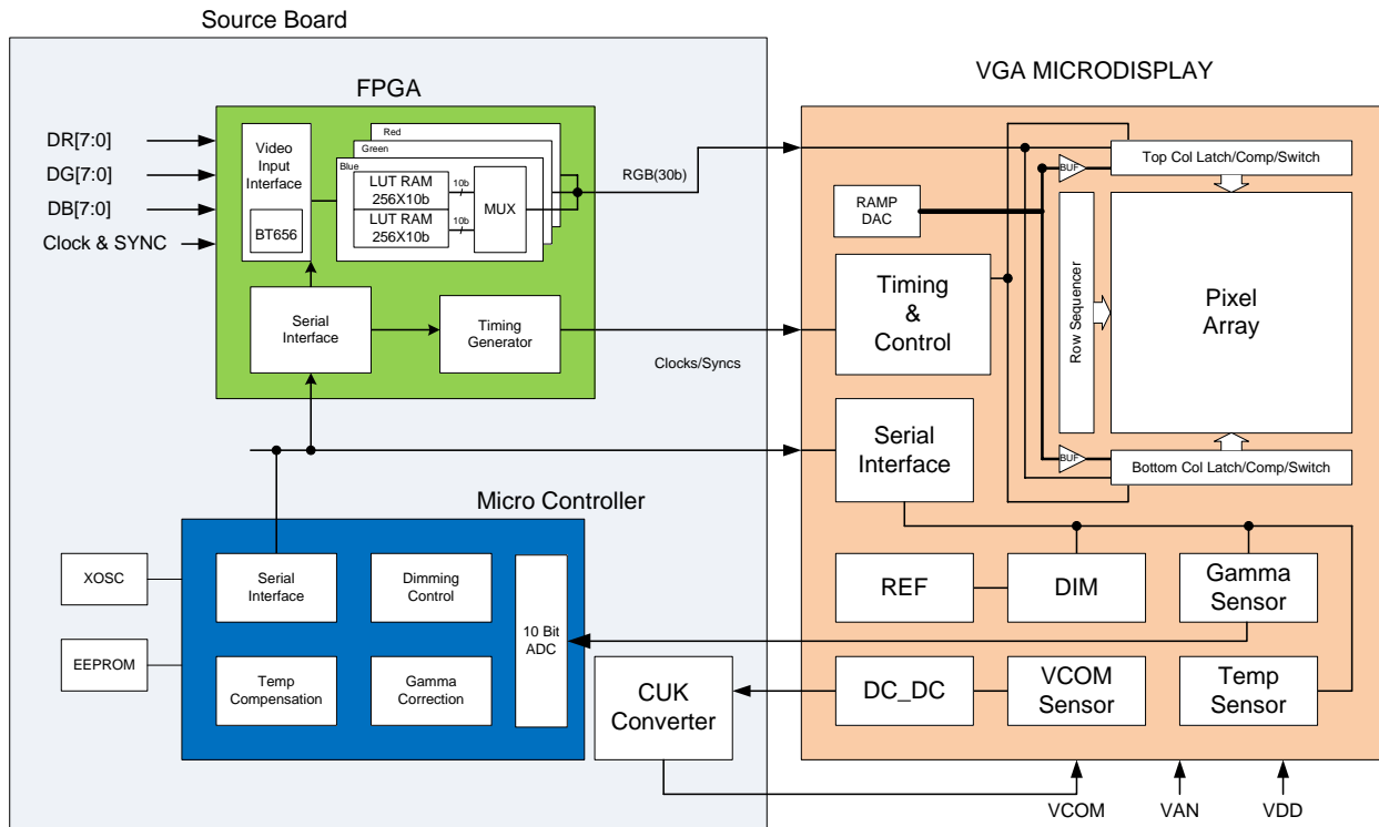
Figure 19: Block diagram of application reference system
