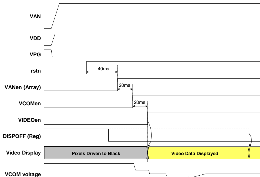
Figure 15 : Power-Up sequence for supplies and control.
