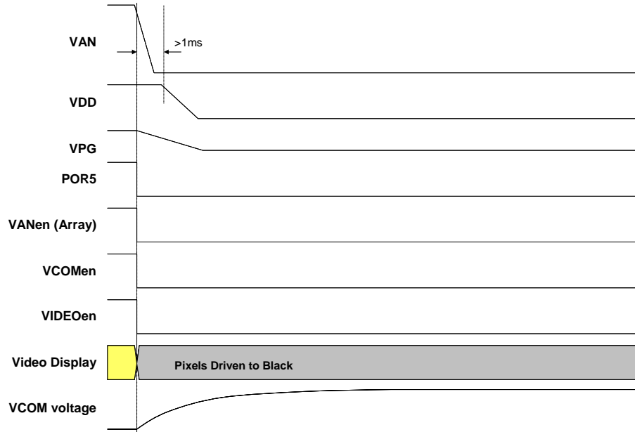
Figure 17: Power-Down sequence for supplies and control.
