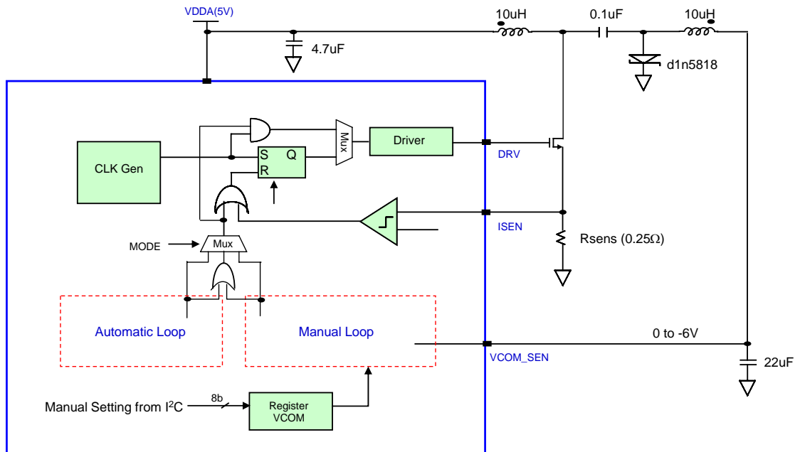
Figure 13 : Schematic of DC-DC controller function
