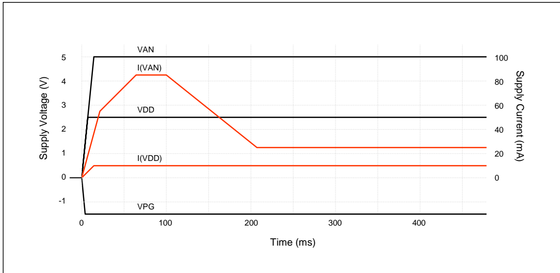
Figure 16: Typical startup currents
