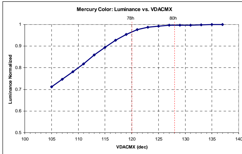
Figure 19: Luminance dependency on VDACMX
