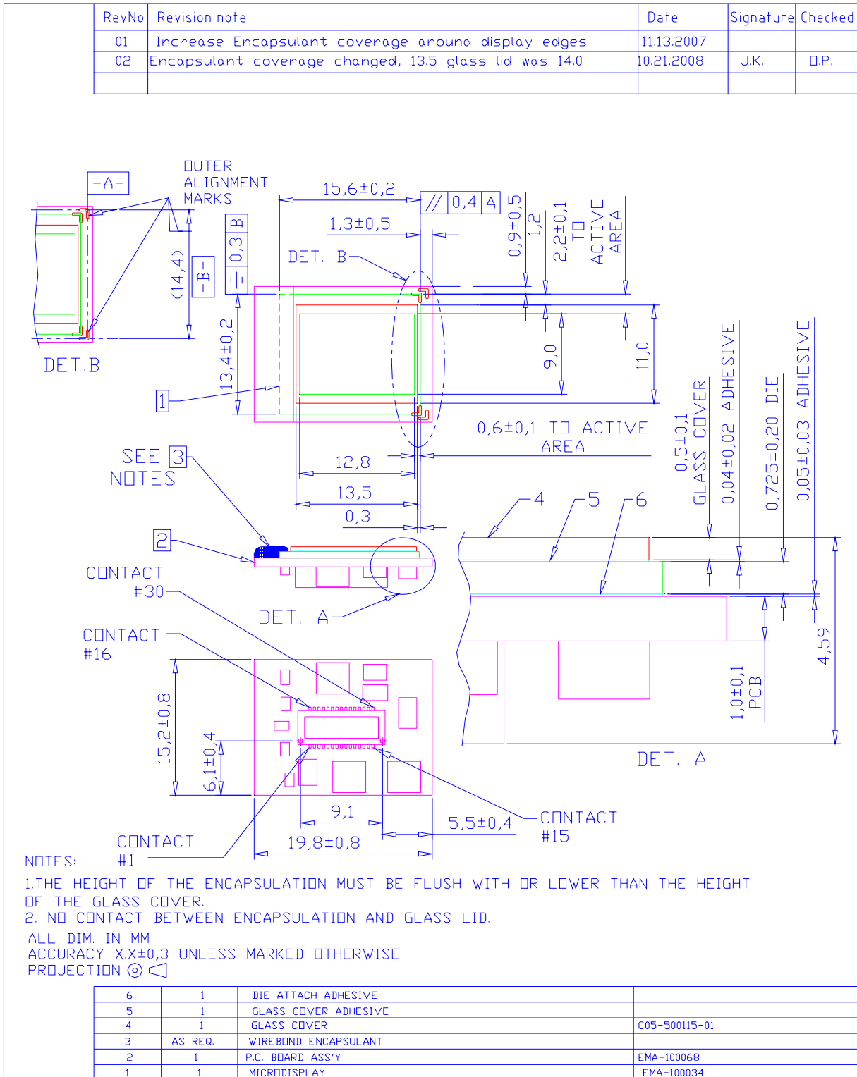
Figure 7-1. Mechanical Characteristics
